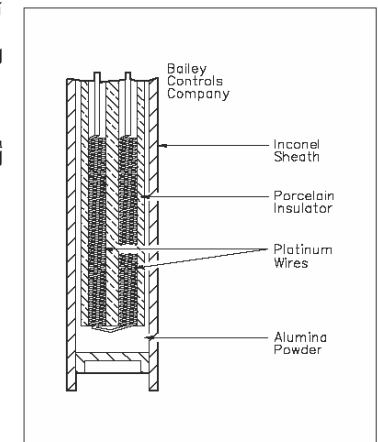
Figure 2 Internal Construction of a Typical RTD
