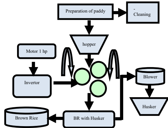
Fig. 2 Diagram of brown rice peeling machine
